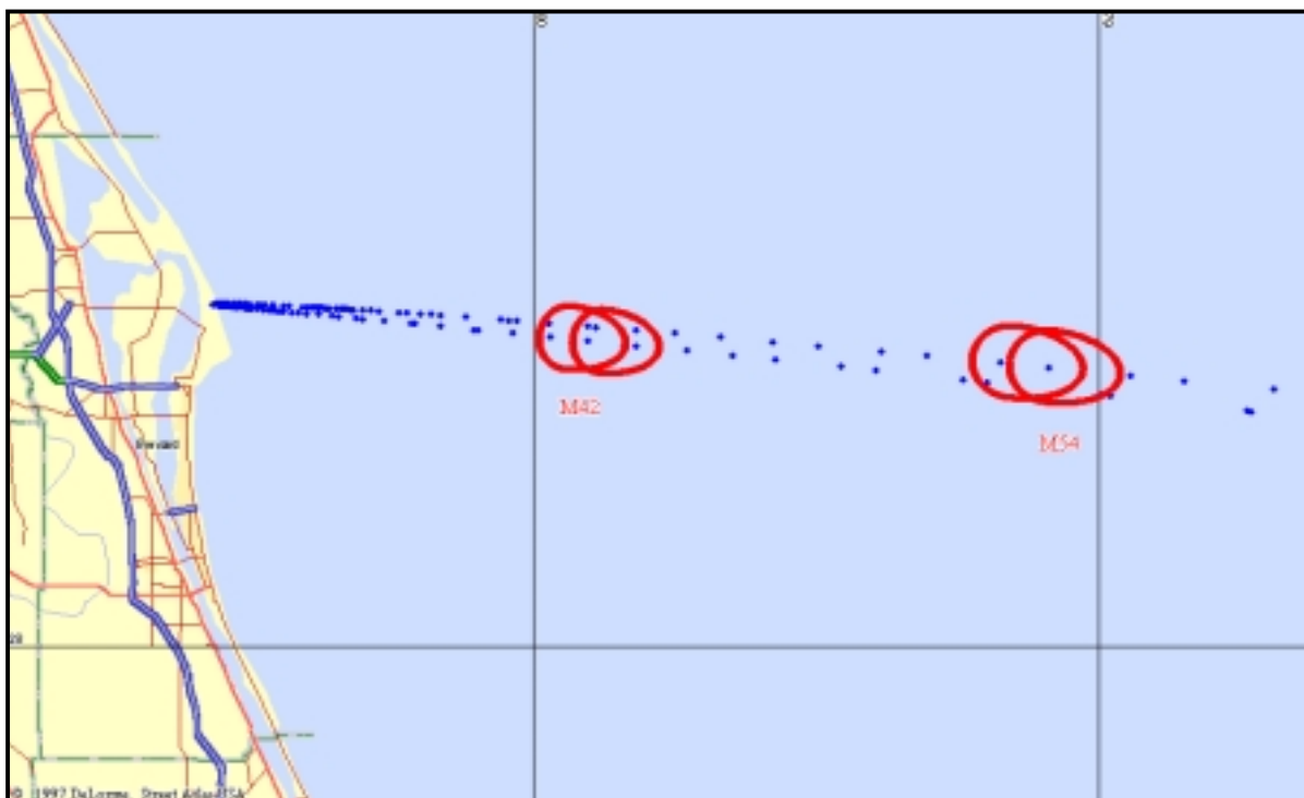
Estimated Solid Motor Impact Ellipses Delta IV-M42 and M54 GTO and LEO Launches
