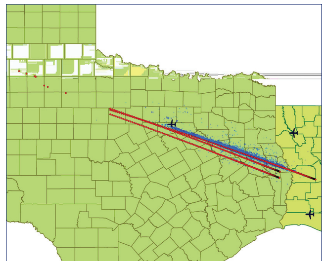
Figure 2-7. Reference Trajectories.
