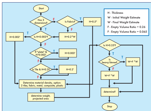
Figure 2-5. Rule Based \beta (Ballistic Coefficient) Approximation.
