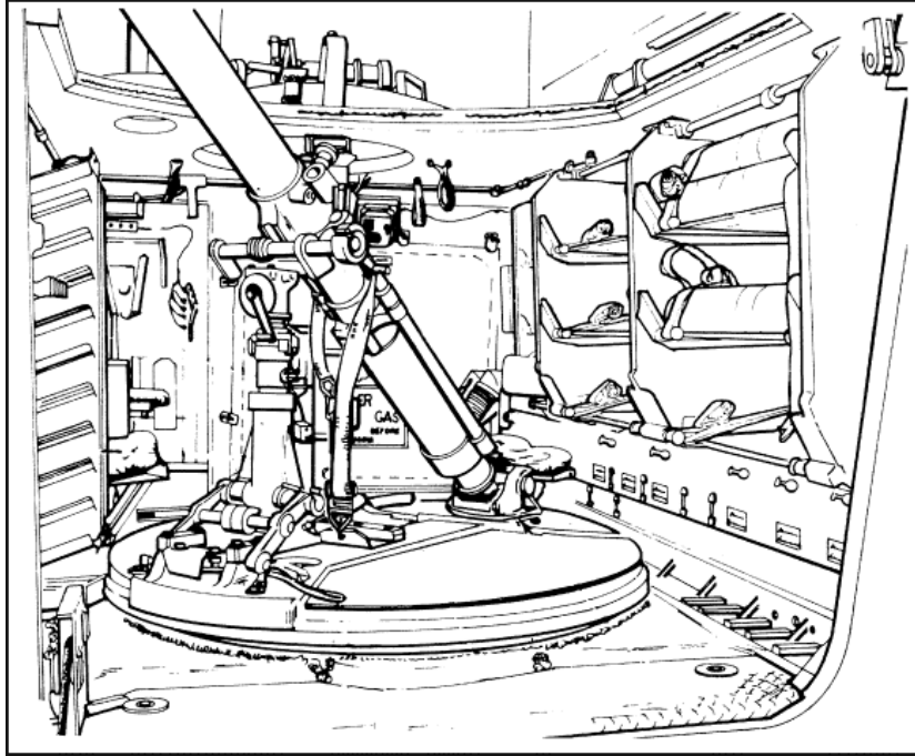
Figure 6-18. Vehicular mount.
