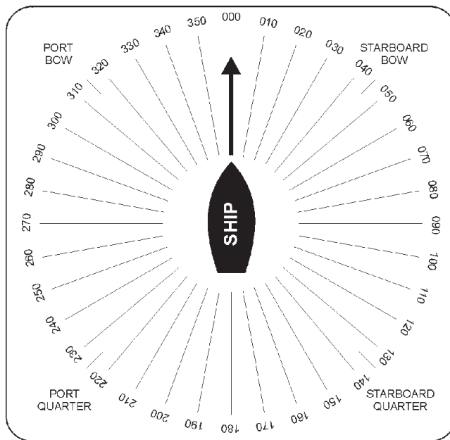
Figure 3-2.—Relative bearings.
